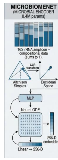
Figure 4. MicroBiomeNet microbial encoder (8.4M parameters). 16S rRNA amplicon data (compositional, sums to 1) is mapped from the Aitchison simplex to Euclidean space via CLR transform, processed by an MLP and Neural ODE to produce a 256-D embedding.
